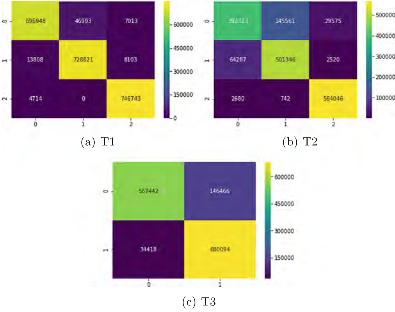
Fig. 3. Confusion matrices.
