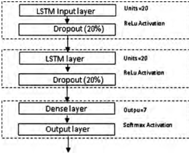
Fig. 1. LSTM development.
