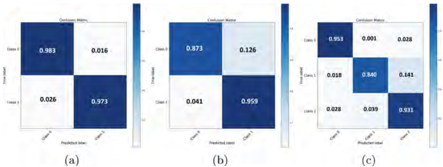
Fig. 4. Confusion matrix of leave-one-subject-out hierarchical sleep stages classification utilizing posture data knowledge (a) Training phase, Class 0: Wake, Class 1: Sleep (b) Training phase, Class 0: REM, Class 1: NREM (c) Hierarchical testing phase Class 0: Wake, Class 1: REM, Class 2: NREM
