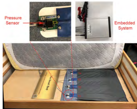
Fig. 1. Hydraulic bed sensor system.
